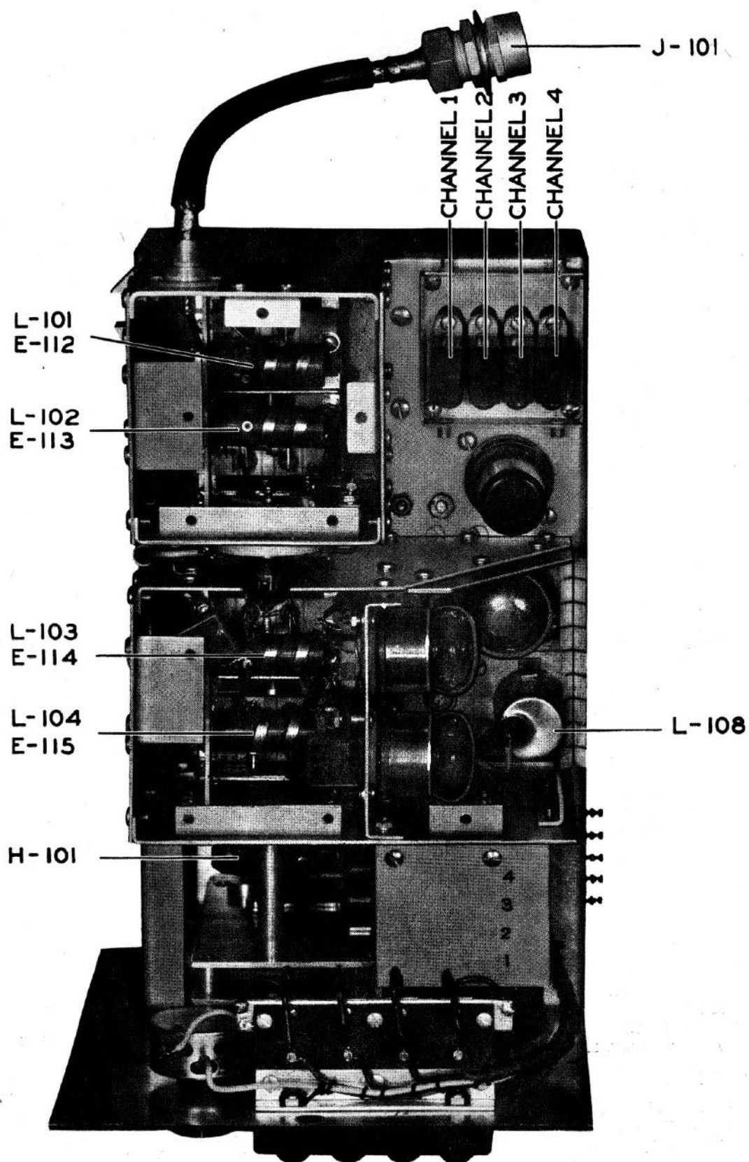
Figure 2.121 TOP VIEW OF PRESECTOR UNIT
