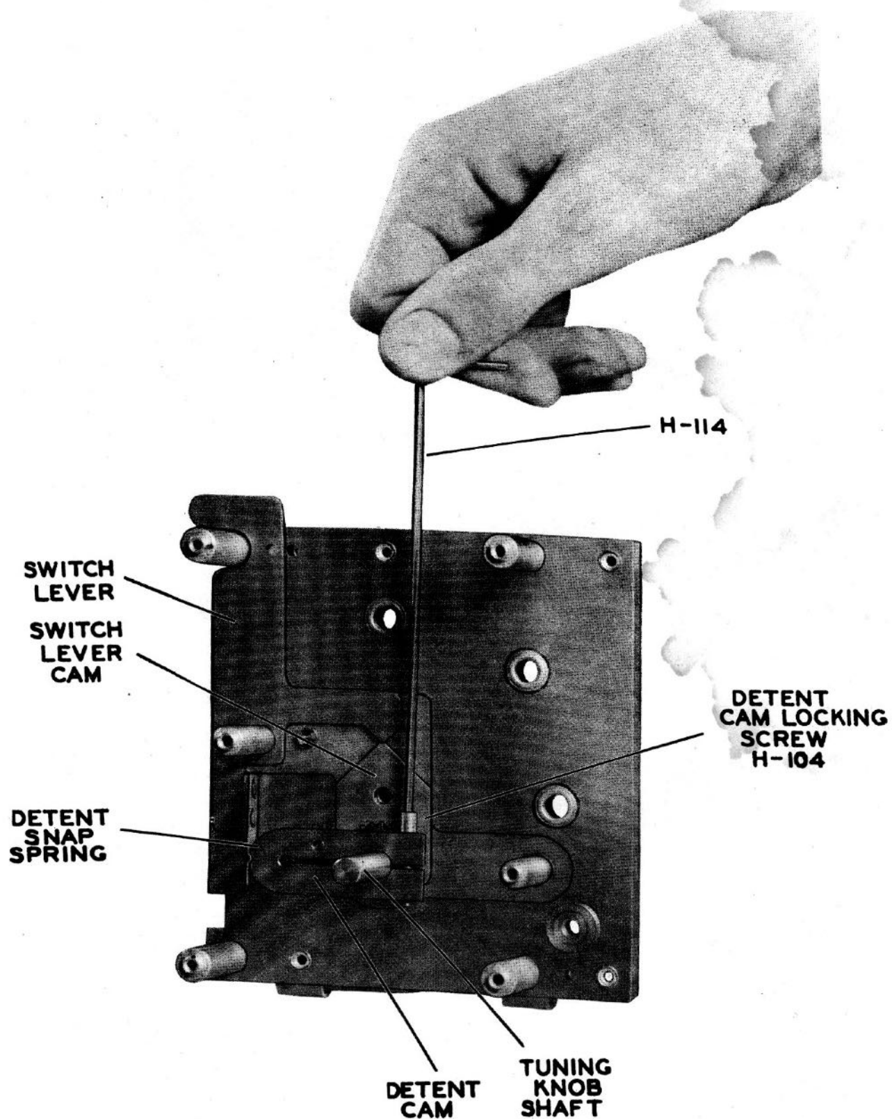
Figure 4.21B CUTAWAY MODEL SHOWING THE SETTING OF ONE DETENT POSITION
