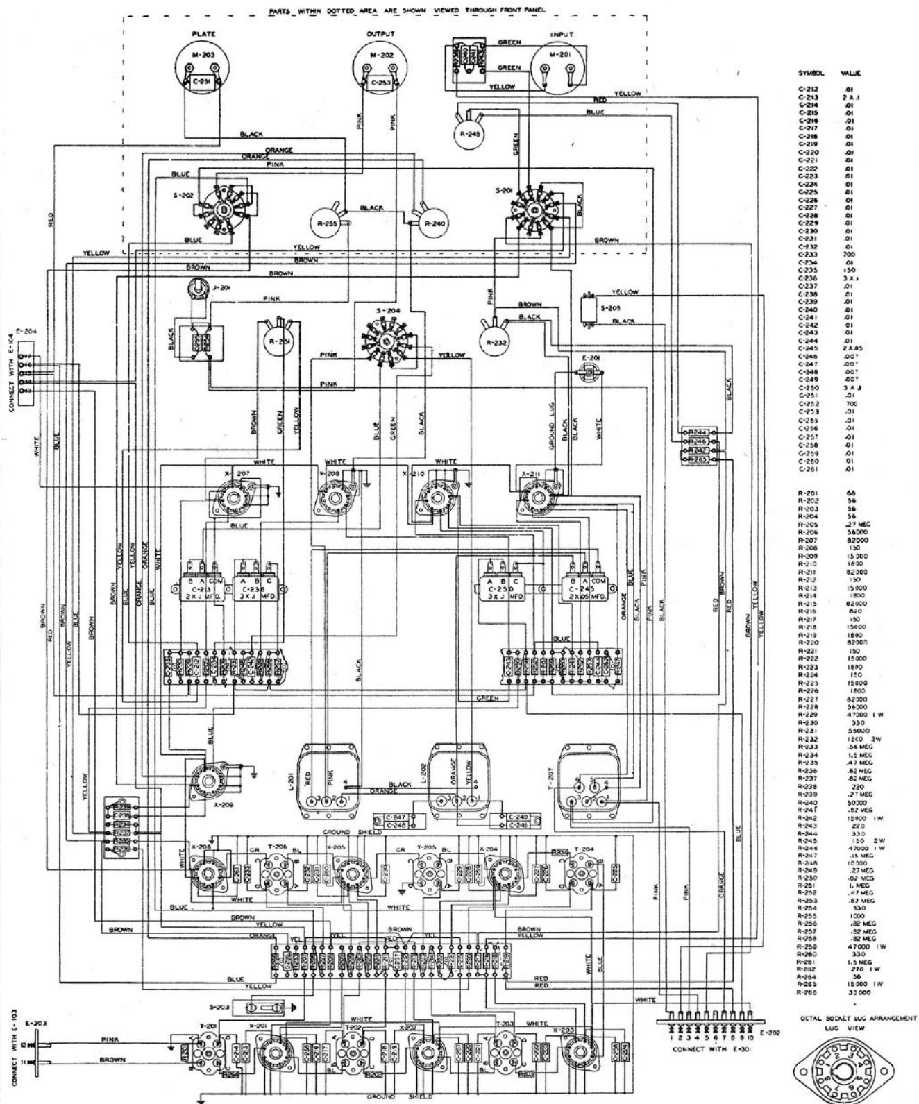
Figure 8.2 I-F/A-F CHASSIS WIRING DIAGRAM
